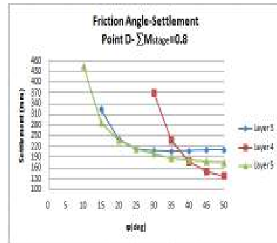
Figure 8: Subsidence changes with changes in coefficient of internal friction layer for D point
