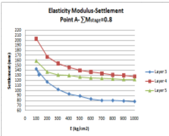
Figure 5: Changes in the subsidence of A point
