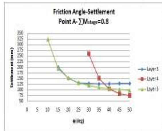
Figure 7: Subsidence changes with changes in coefficient of internal friction layer for A point
