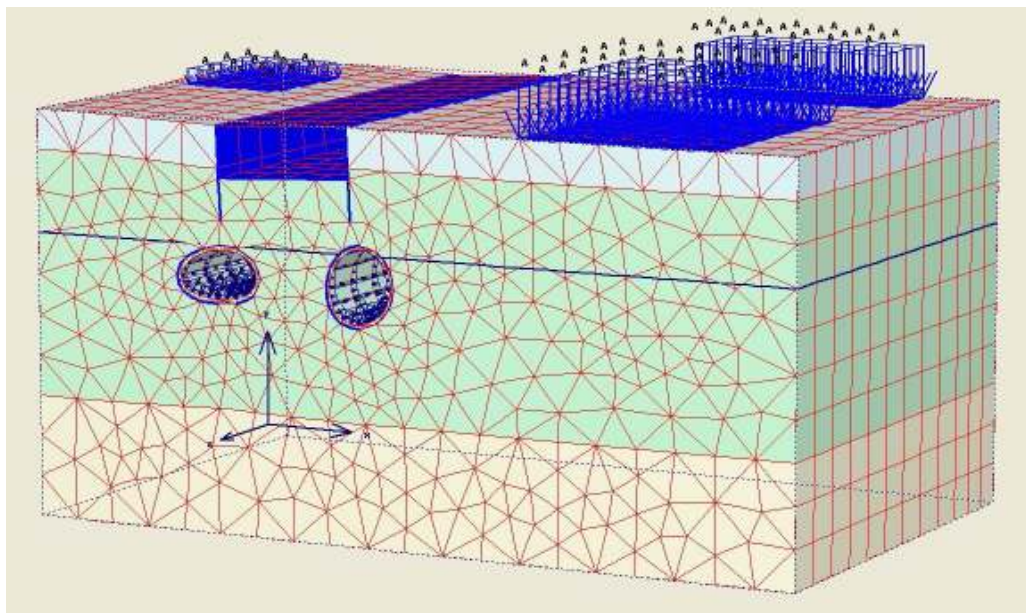
Figure 4: 3D finite element model
