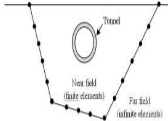
Figure 1: Schematic of the finite/infinite element approach
