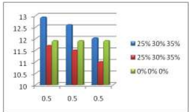
Graph 1. Graph showing compression test values for 7 days of fly ash concrete with varying percentages and ordinary concrete with different water-cement ratios
