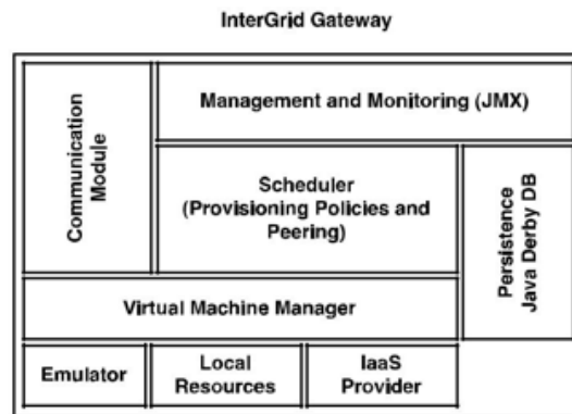
Fig. 2 Main components of the IGG
