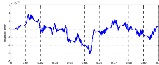
Fig.12.4: Reactive Power loading for Inverter 2
