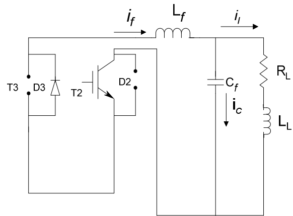
Fig.5 :Conducting State whenT 1 goes Off and D 3 comes in action
