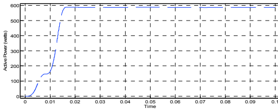
Fig.13.1:Active power loading for Inverter 1
