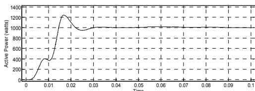
Fig.11.1: Active power loading for Inverter 1
