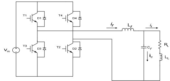
Fig.3: Layout of H-Bridge Inverter
