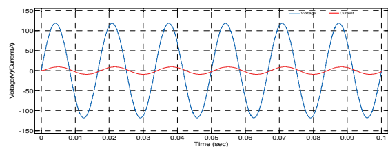
Fig.9.1 :Voltage and current waveform for inductive Load
