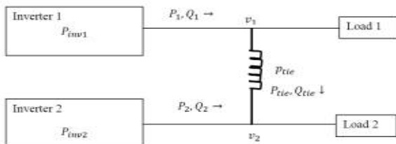
Fig.2 :Two parallel operating inverter with tie-line
