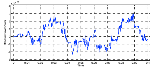
Fig.13.2: Reactive Power loading for Inverter 1
