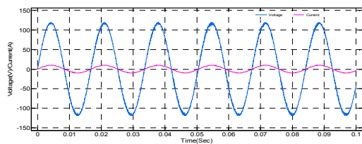
Fig.9.2: Voltage and current waveform for inductive Load
