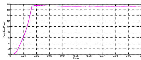
Fig.13.4: Reactive Power loading for Inverter 2
