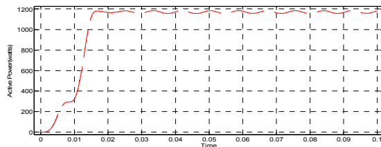
Fig.14.1: Active power loading for Inverter 1
