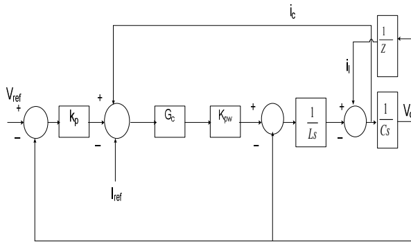
Fig.6 :Represents the control diagram for single unit inverter
