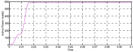
Fig.12.1 Active power loading for Inverter 1
