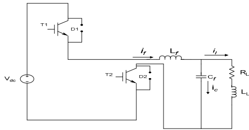
Fig.4 :Conducting State for T 1 and T 2
