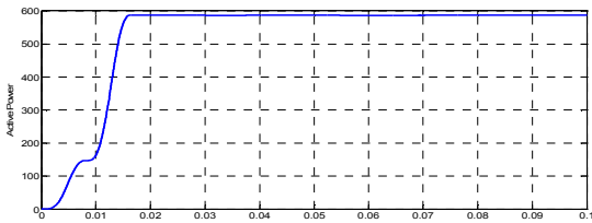
Fig.12.3 :Active power loading for Inverter 2
