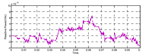
Fig.12.2: Reactive Power loading for Inverter 1
