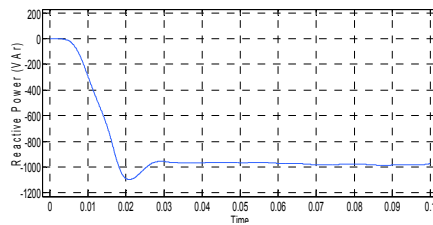
Fig.11.2: Reactive Power loading for Inverter 1
