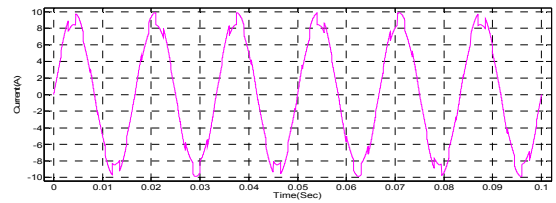
Fig.10.3: Current Waveform during Step change in Load
