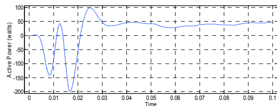
Fig.11.1: Active power loading for Inverter 1
