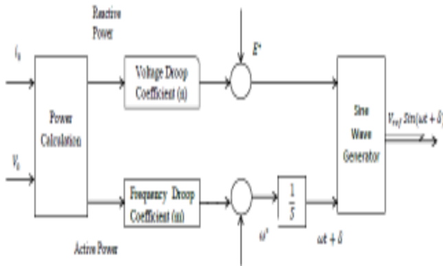
Fig.7 :Traditional Droop Control Schemes for Reference Generation
